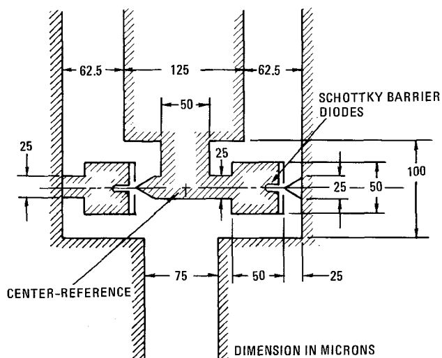
Figure 2. Diode Arrangement at the Magic Tee Junction.
