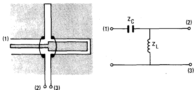
Figure 3. Equivalent Circuit of the Coplanar Stripline/Slotline Transition.
