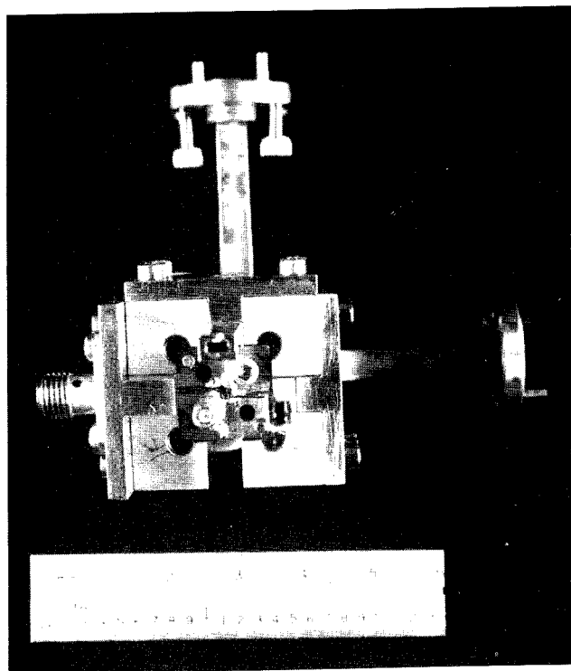
Figure 6. W-Band Monolithic Mixer Test Fixture Assembly.
