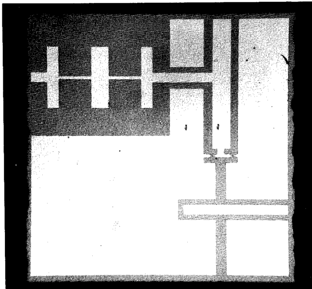
Figure 5. Monolithic GaAs Mixer Chip.
